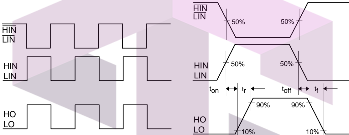
Figure 1. Input/Output Timing Diagram
